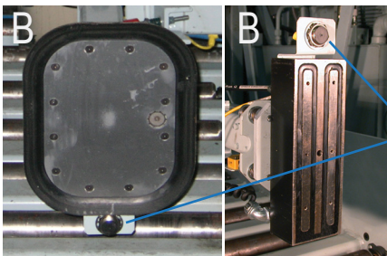
Extractor arm /w magnet or vacuum
