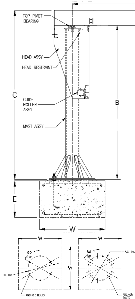
Chart represents a sample of J-904B Sizes & Capacities
